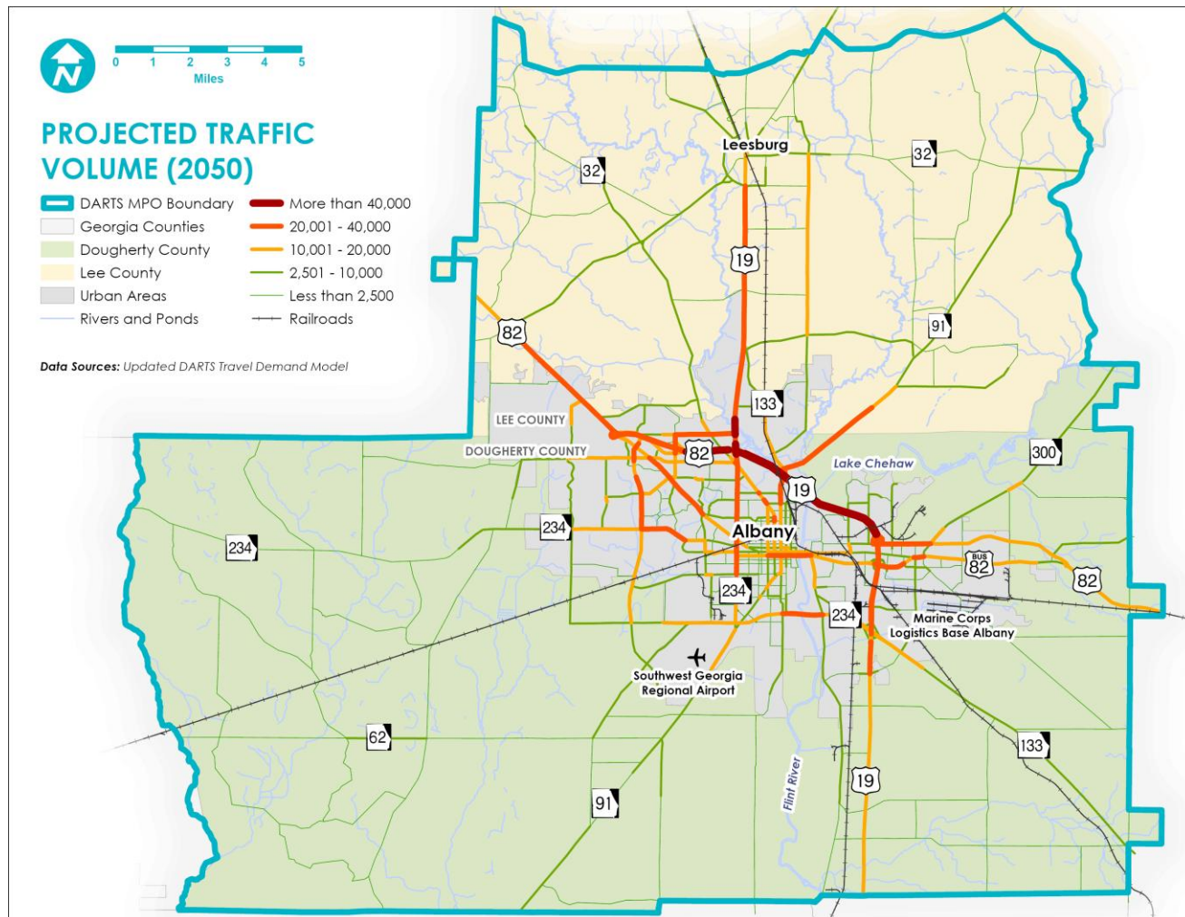
Figure 8-8: 2050 E+C Traffic Forecasts
